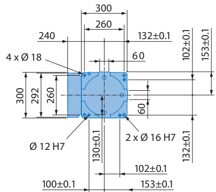
Mounting options: Floor, ceiling, wall
